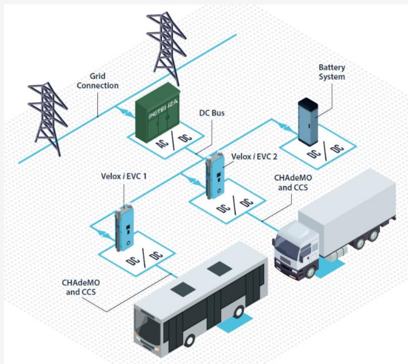
Figure 1 - A typical Velox / Ultra Rapid charging system arrangement
