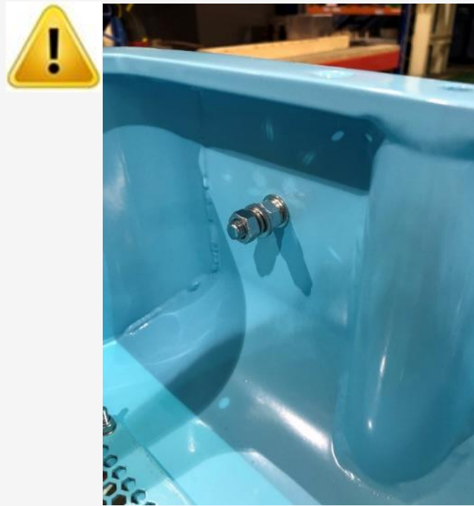
Figure 20 - PE Connection
