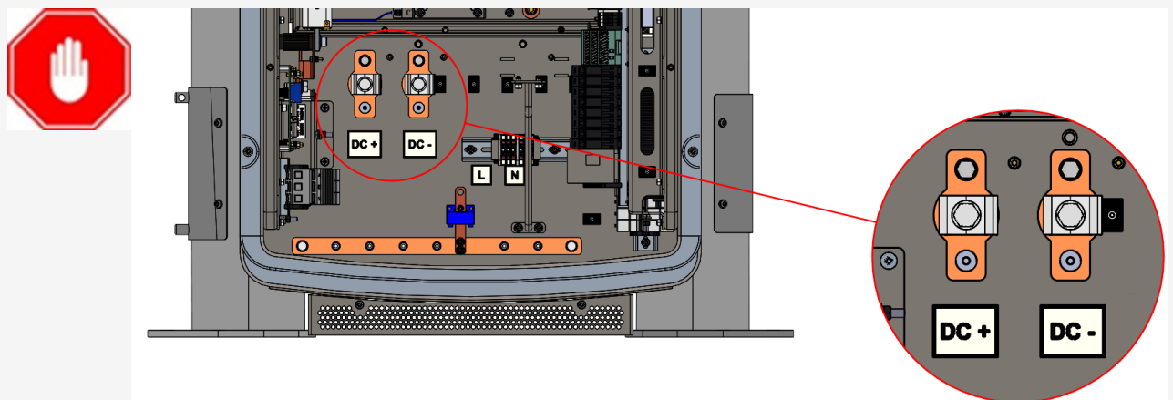
Figure 14 - DC input terminal connection details
